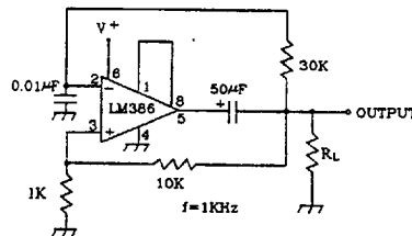
Square Wave Oscillator
