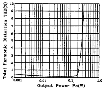
Total Harmonic Distortion vs. Output Power (V + =6V, R L =8Ω, f=1KHz)
