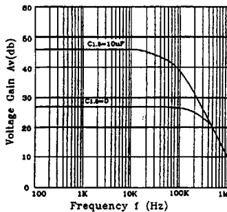
Voltage Gain vs. Frequency
